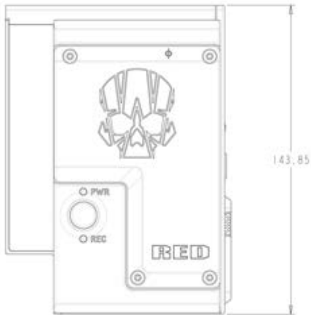
Figure: Camera Side View (Left)
