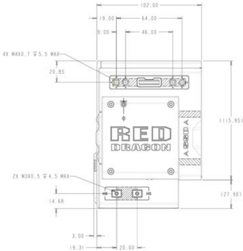
Figure: Camera Side View (Right)
