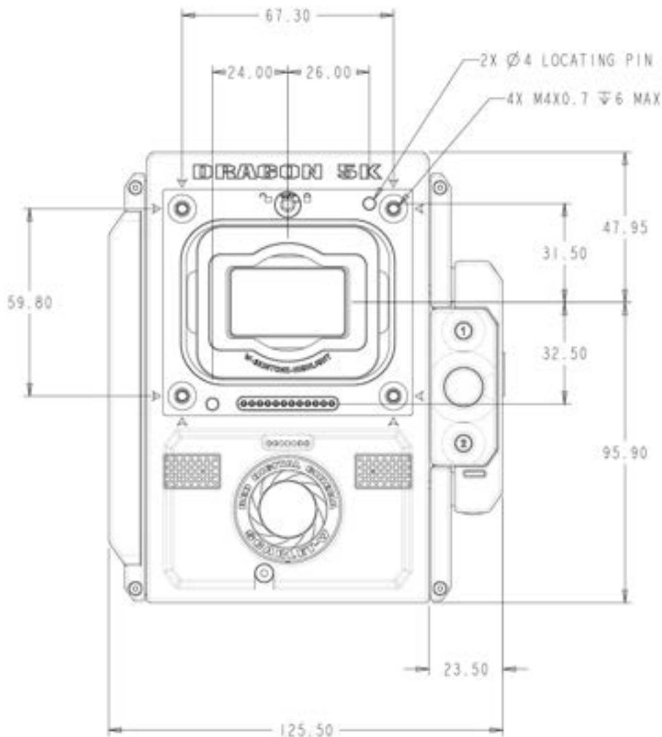
Figure: Camera Front View
